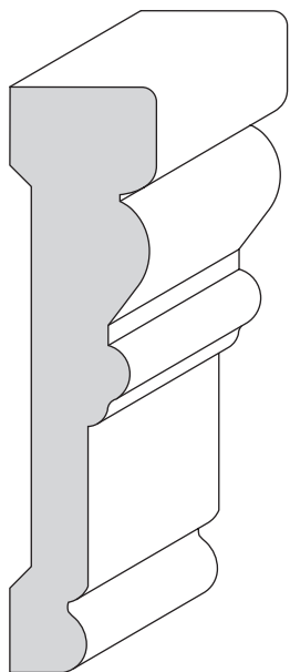
245 11/16 x 2 3/4 Classic Casing
