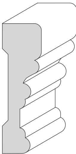
255 11/16 x 2 1/4 Beaded
