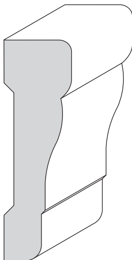
250 11/16 x 2 1/4 Colonial
