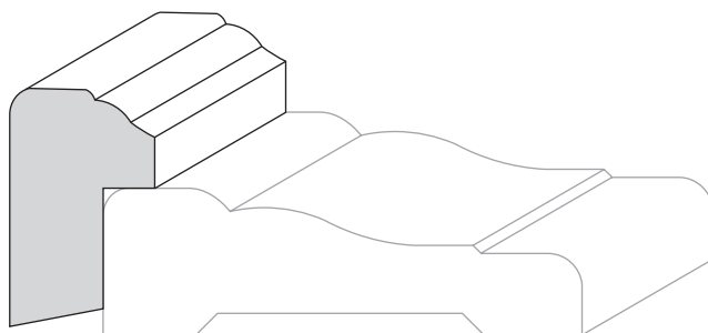
260 11/16 x 1 1/8 Back Band
