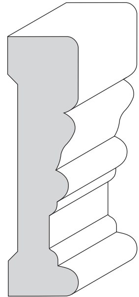
240 3/4 x 2 3/4 Beaded
