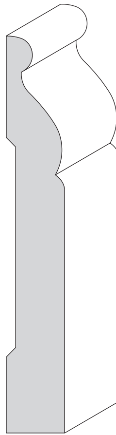
330 5/8 x 4 1/4 Modified
