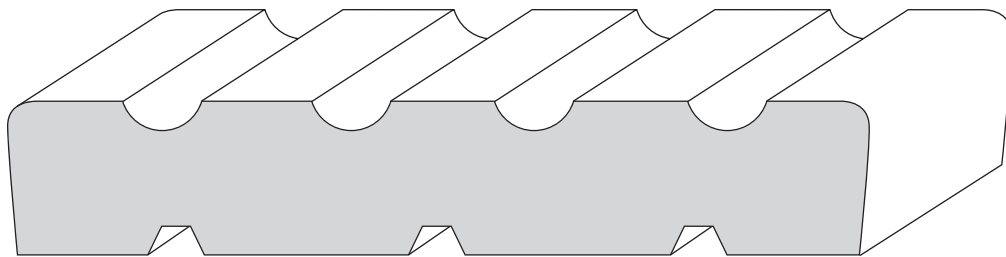
680 • 3/4 x 4 9/16 x 81 3/4 • Fluted Door Jamb (Fluted 8" from bottom, 6" from top)
